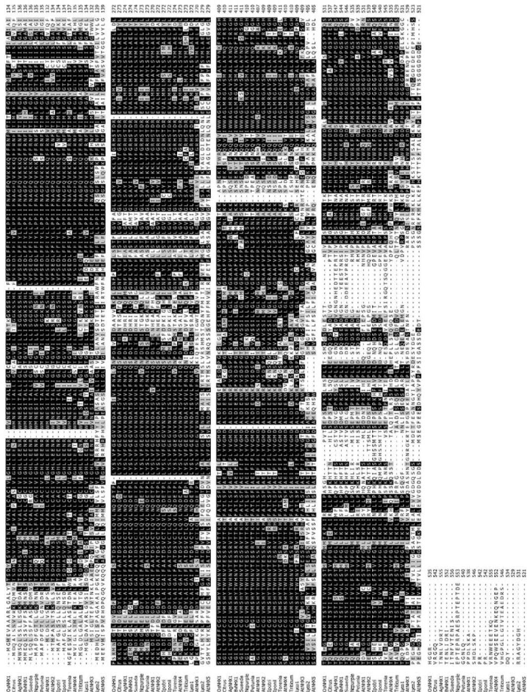
Figure 1. Alignment of full-length NHX-like proteins. Titles in the alignment correspond to accession numbers and species as follows: AgNHX1, BAB11940, Atriplex gmelini ; AINH1, AAD16946, Arabidopsis thaliana ; AINH2, AAG51408, A. thaliana ; AINH3, BAB08564, A. thaliana ; AINH4, AAF08577, A. thaliana ; AINH5, A. thaliana ; AINH6, AAD25617; Citrus, AAK27314, Citrus x paradisi ; Iponil, BAB16380, Ipomoea nil ; Ipotri, BAB60901, Ipomoea tricolor ; Lyco1, CAC84522, Lycopersicon esculentum ; Nepurple, BAB56106, Nierembergia caerulea ; OSNHX1, BAA83337, Oryza sativa ; Petunia, BAB56105, Petunia x hybrida ; Suaeda, AAK53432, Suaeda maritima subsp. Salsa; Torenia, BAB56107, Torenia hybrida ; Triticum, AAK76737, Triticum aestivum . Residues in black are identical; residues in grey are conservative substitutions.
